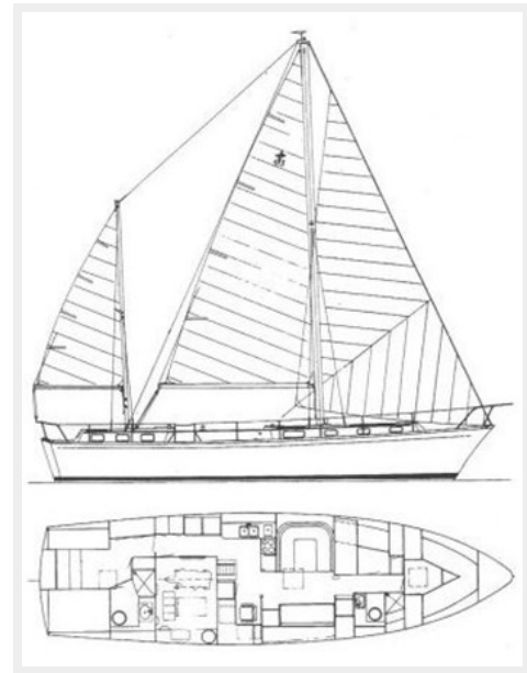
110 gulfstar_53_ms_drawing
