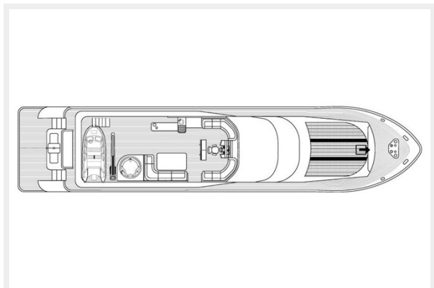
MIA KAI Bilgin Tiago 100 - Main Deck layout.
