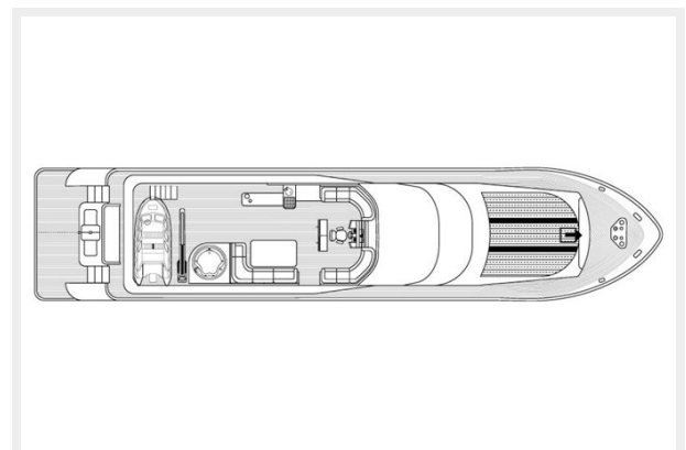
MIA KAI Bilgin Tiago 100 - Main Deck layout.
