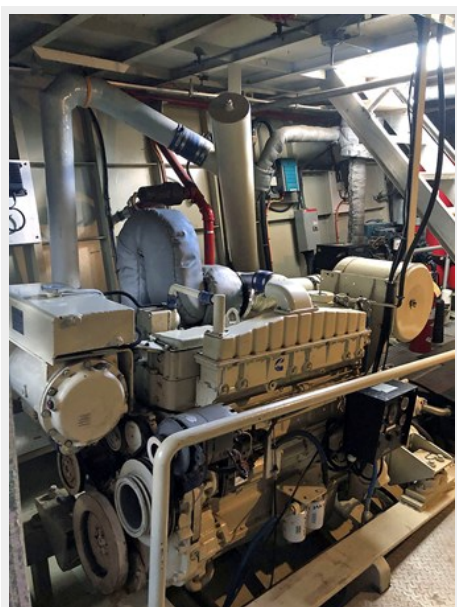
Chagos_stb_engine_looking_aft
