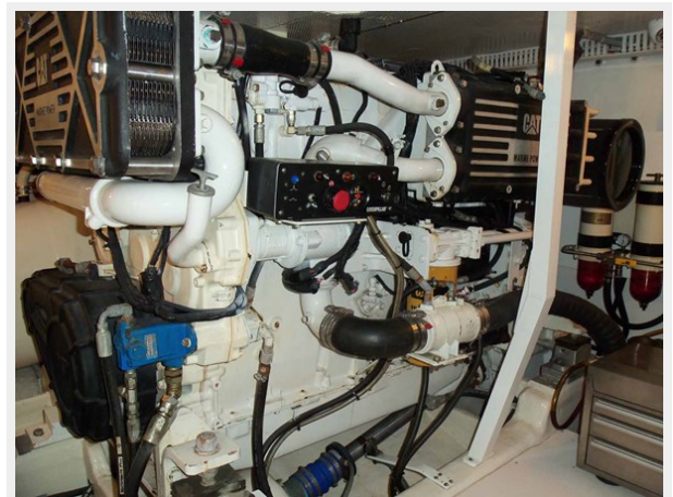
Port Engine
