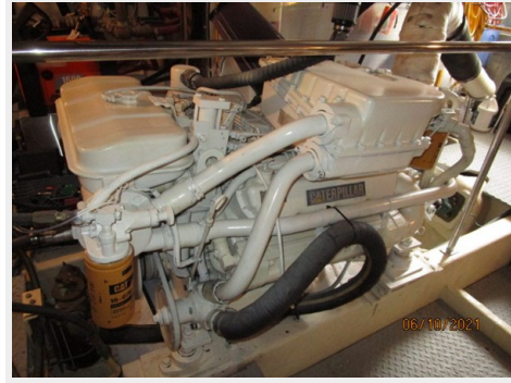
51_2780267_55_symbol_starboard_main_engine
