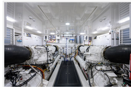
92_viking_completely_knots_engine_room_1
