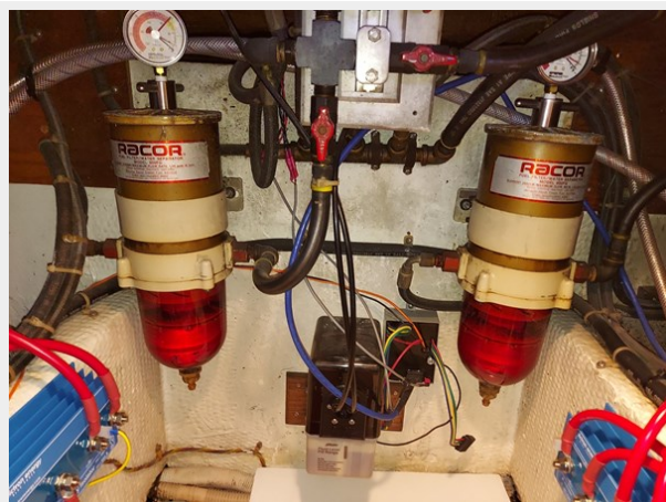
0133 Engine Room
