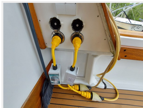
0049 shore power
