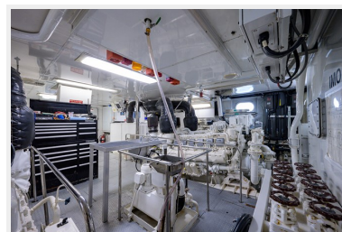
136_intermarine_burgas_engine_room_16
