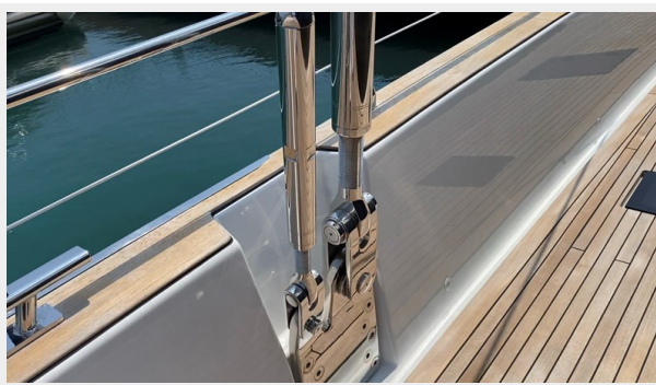
Impressive chainplate
