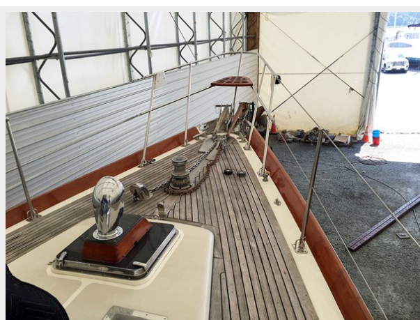
Foredeck, Fwd.
