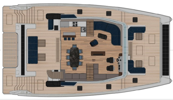
MAIN DECK
