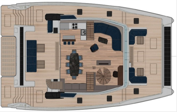
OPTIONAL - MAIN DECK CONFIGURATION FOR ENCLOSED SKYLOUNGE
