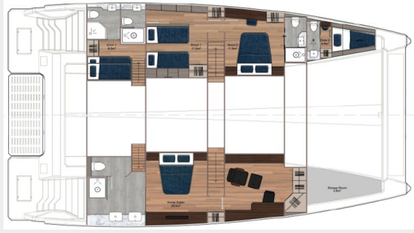
LOWER DECK - Owner Version
