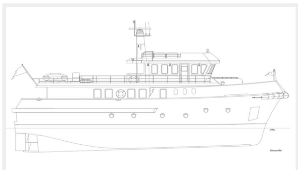
yacht-akula-24m-GA-02
