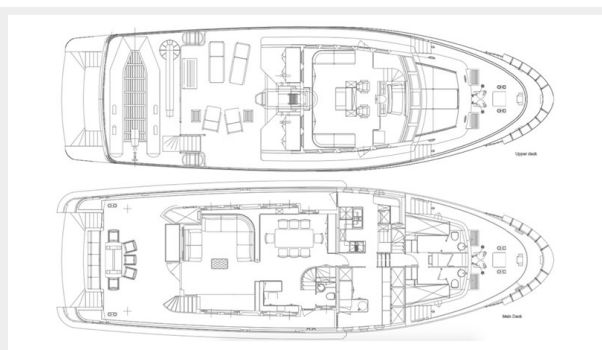
yacht-akula-24m-GA-01
