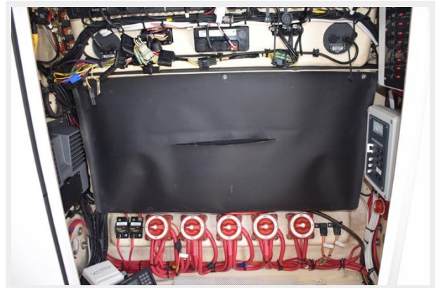
Radial battery switches - access to electronics
