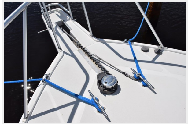
Electric windlass and pulpit with roller chute
