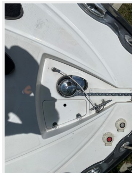
10-Windlaass
