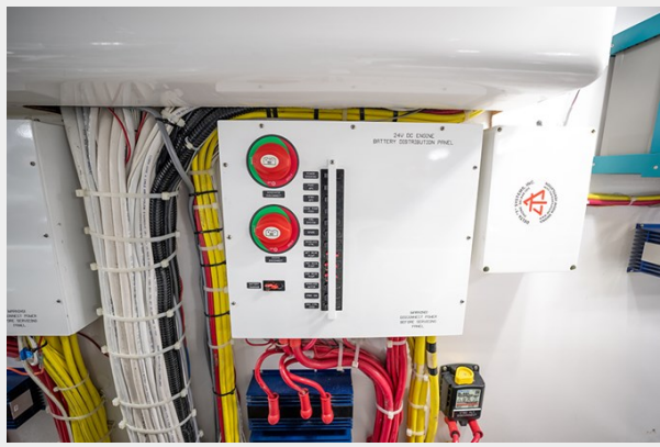
Battery distribution panel
