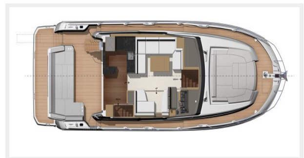
PRESTIGE-590---Main-Deck---Relax-cockpit- -800px
