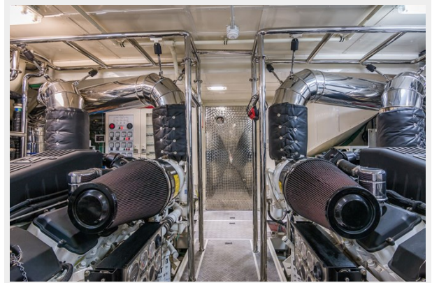
PRIMA MEA 107'/32.61m Vicem 2013/2021: Engine Room
