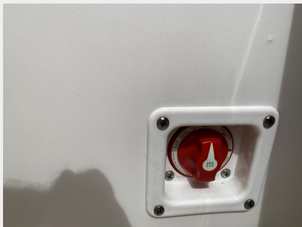
18-BATTERY SWITCH
