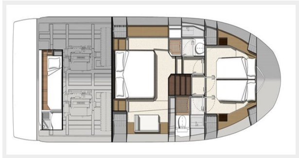
Cabin layout (002)
