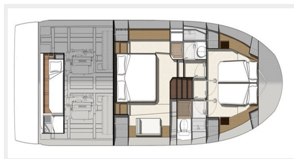
Cabin layout (002)
