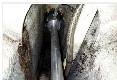
48_2790410_1048_wandering_star_dripless_shaft_seal
