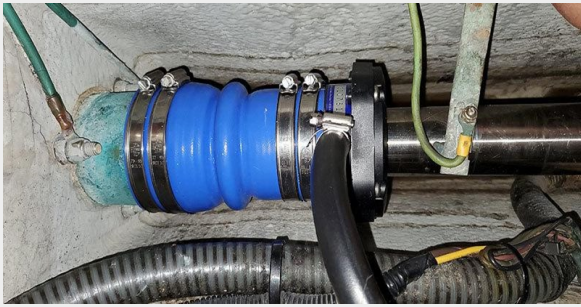
41_2790446_dripless_shaft_seal
