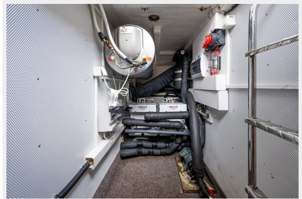
56_galeon_the_dream_engine_room_6 56_galeon_the_dream_engine_room_7
