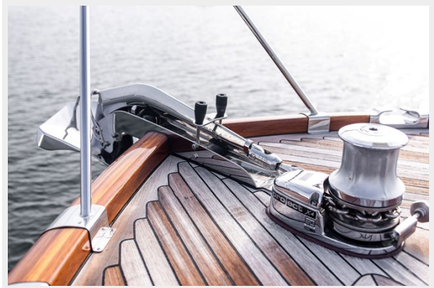
Anchor Windlass
