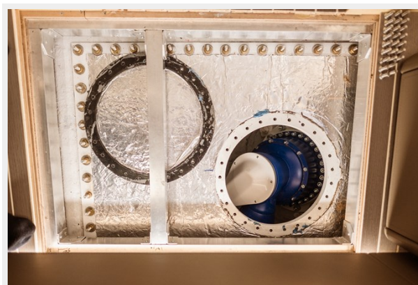
Cofferdam System
