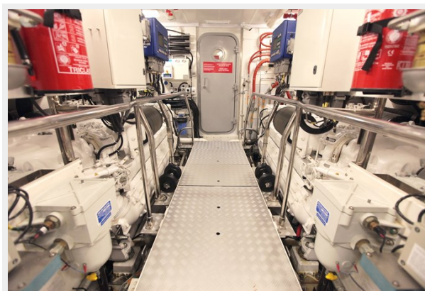
Princess_32M-ref.015_Engine_2
