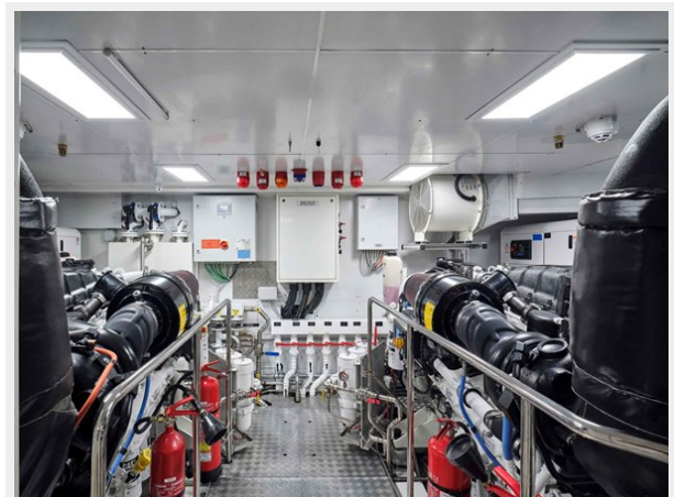
Navetta Custom Line 42 Engine Room
