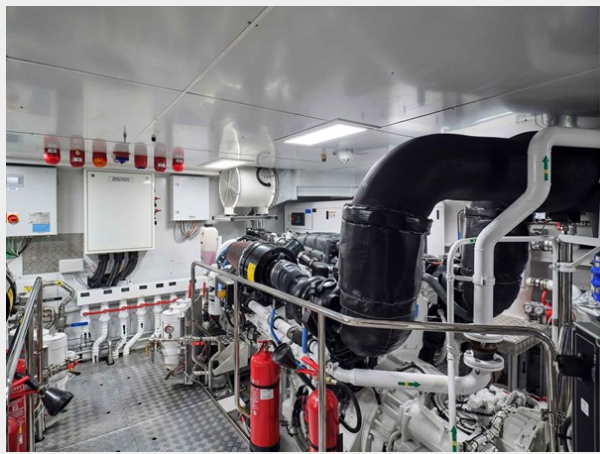
Navetta Custom Line 42 Engine Room
