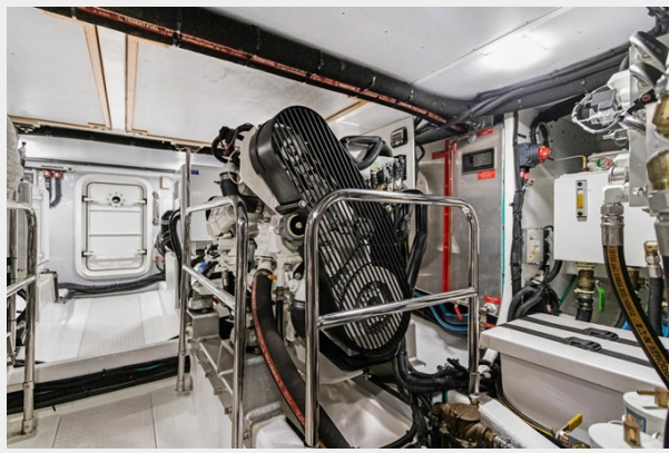
Port engine
