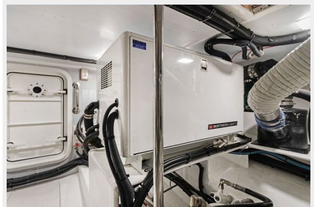
Generator port side aft
