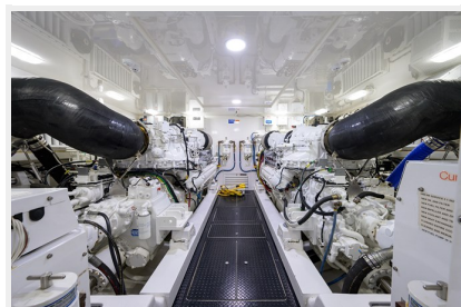
80_viking_eb_set_in_my_waves_engine_room_1
