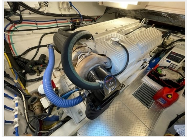
2007 TIARA 4700 SOVRAN stbd engine picture
