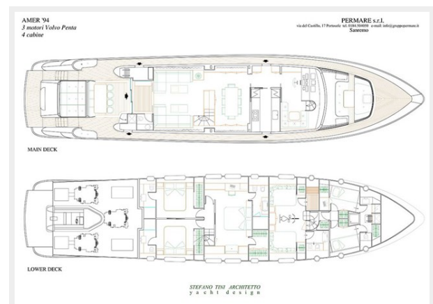
Layout Drawing
