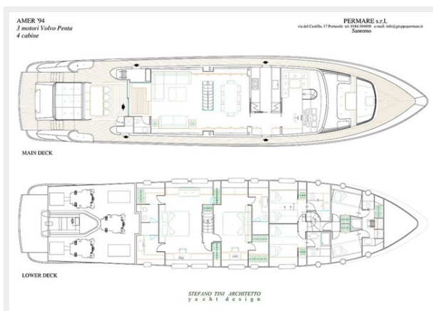
Layout Drawing
