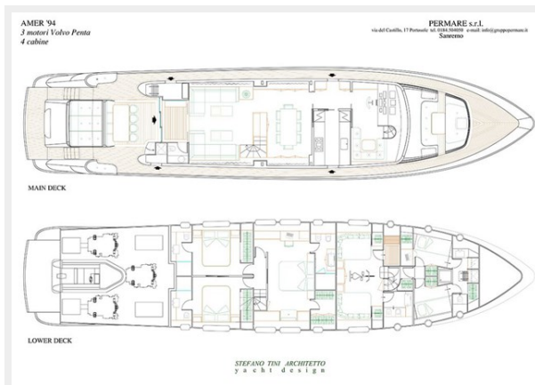
Layout Drawing
