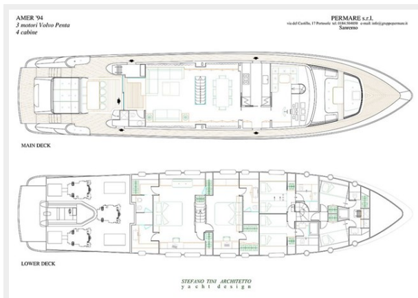
Layout Drawing
