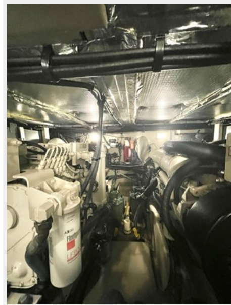
77 Archimedes II 2004 Sea Ray 390 MY Engine Room 4
