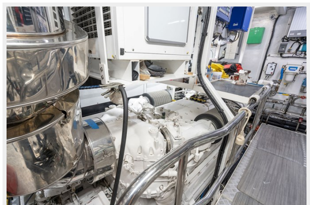
Port Engine
