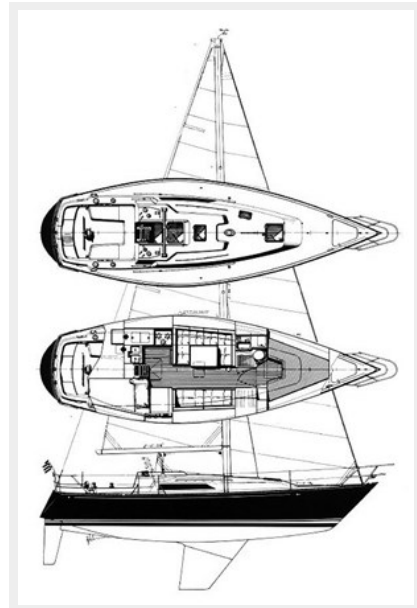
c&c_35-III_drawing
