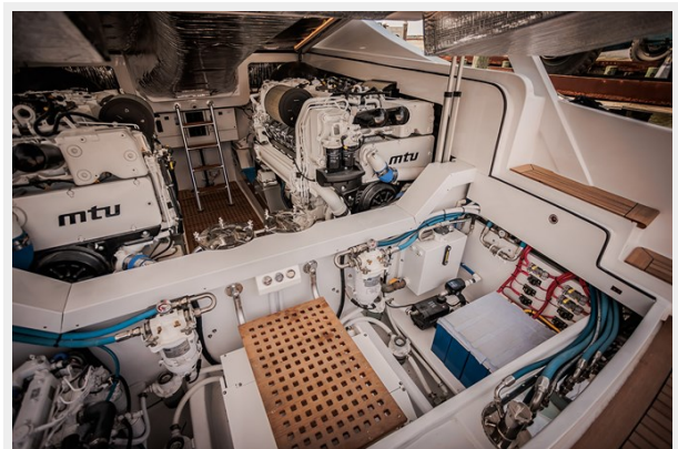
CY55 Machinery Space
