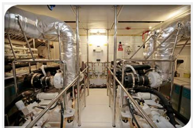
Trader super 70-engine room
