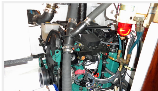
Main Engine
