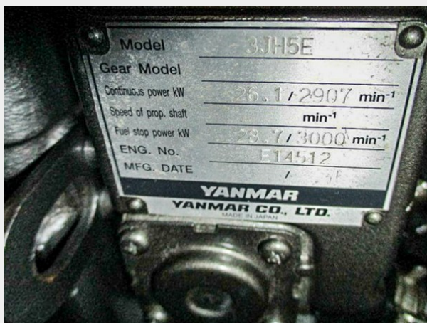
122_2799724_engine_plate
