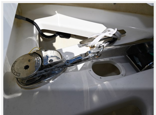
19 Bow electric Lewmar anchor system
