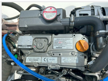
49_2800129_miss_baker_2017_ranger_tugs_r_21ec_yanmar_engine
