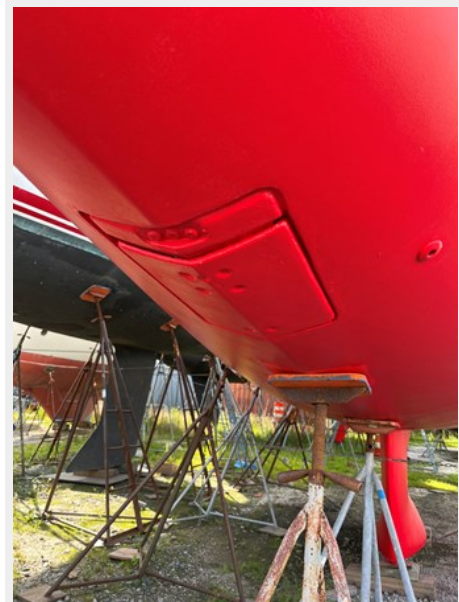
Retractable Bow Thruster
