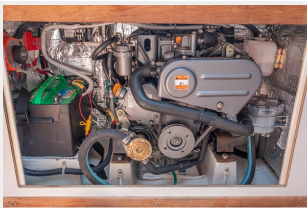
Engine
