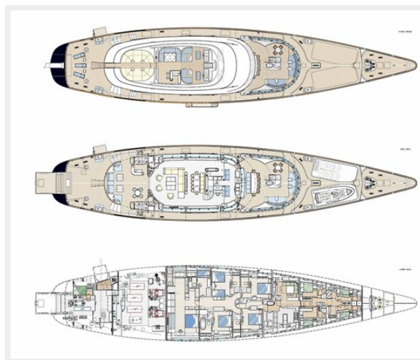
baysian ga
