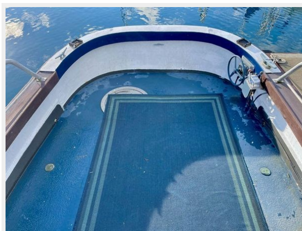
Stockland 36 Trawler Conversion - Cockpit
