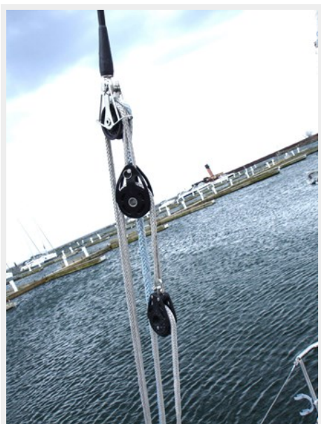
Backstay adjustor cascade DSC08775
